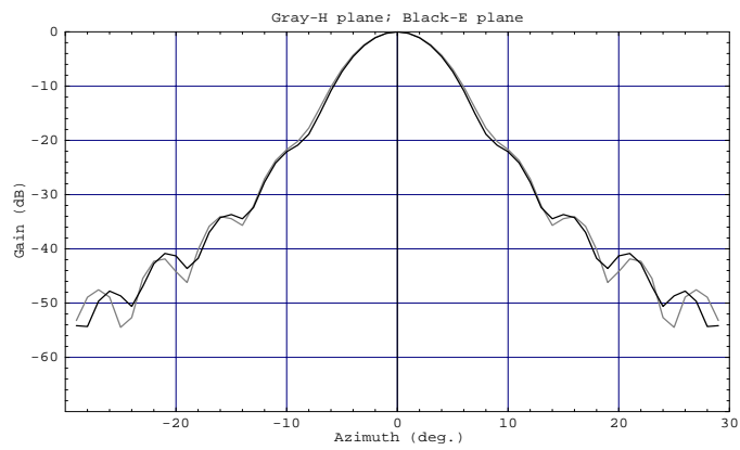
(c) 720 GHz
