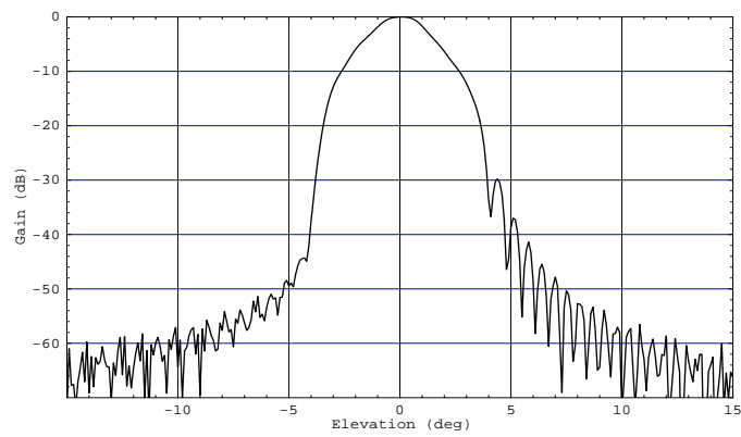
(c) 720 GHz
